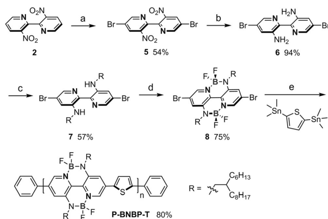
Scheme 3. Synthesis of P-BNBP-T. Reagents and conditions: a) HBr, CH 2 Cl 2 and then Br 2 , 150 °C; b) SnCl 2 ·2H 2 O, HCl, 100 °C; c) n BuLi, THF, -78 °C, then 1-iodo-2-hexyldecane, from -78 °C to 65 °C; d) BF 3 ·Et 2 O, Et 3 N, CH 2 Cl 2 , 50 °C; e) [Pd 2 (dba) 3 ], P( o -Tolyl) 3 , toluene, 120 °C, then bromobenzene.
