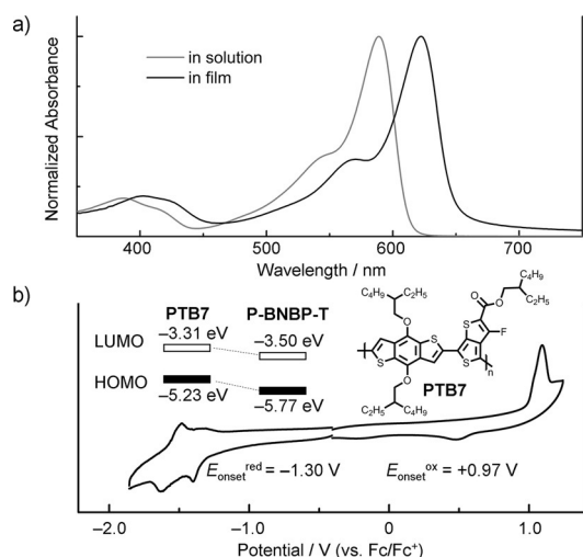
Figure 3. a) UV/Vis absorption spectra of P-BNBP-T in \text{CHCl}_3 solution and in film; b) Cyclic voltammogram of P-BNBP-T in film. Fc = ferrocene. Insets: Schematic of the energy level alignments of P-BNBP-T and PTB7, and chemical structure of PTB7.
