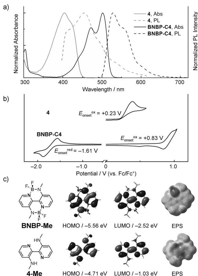
Figure 2. a) UV/Vis absorption spectra and fluorescence spectra of BNBP-C4 and 4 in CHCl 3 solutions; b) Cyclic voltammograms of BNBP-C4 and 4 , Fc = ferrocene; c) LUMO/HOMO and energy levels, as well as electrostatic potential surface (EPS) maps at the 0.0004 electron density of the model compounds BNBP-Me and 4-Me .
